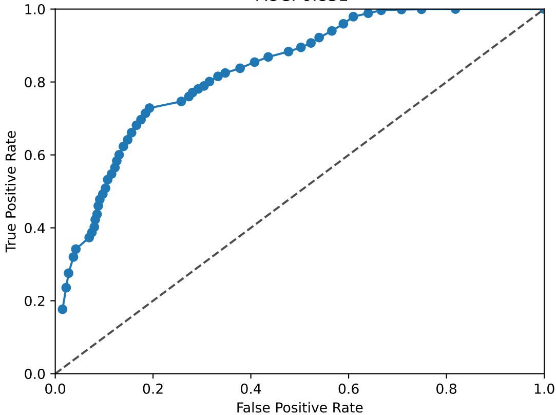
RORA_RORB ROC Curve AUC: 0.831
