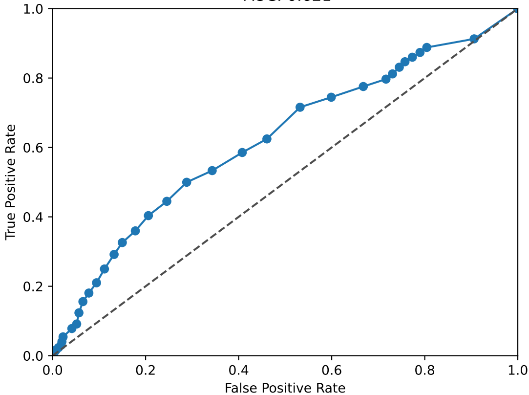
SIX1 ROC Curve AUC: 0.621
