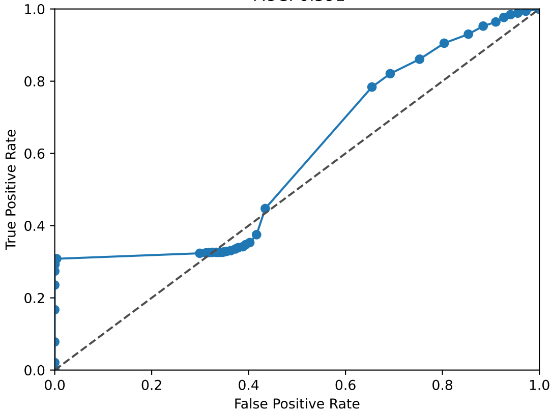
EHF ROC Curve AUC: 0.591
