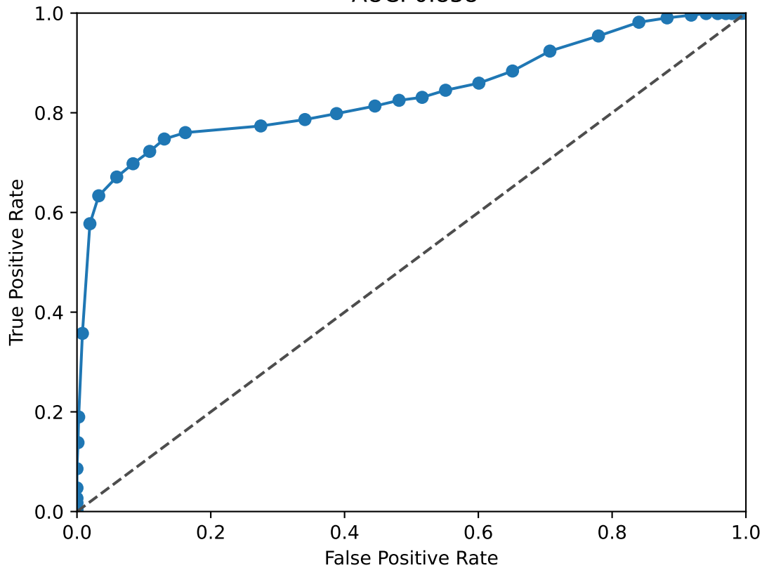
FOS ROC Curve AUC: 0.838
