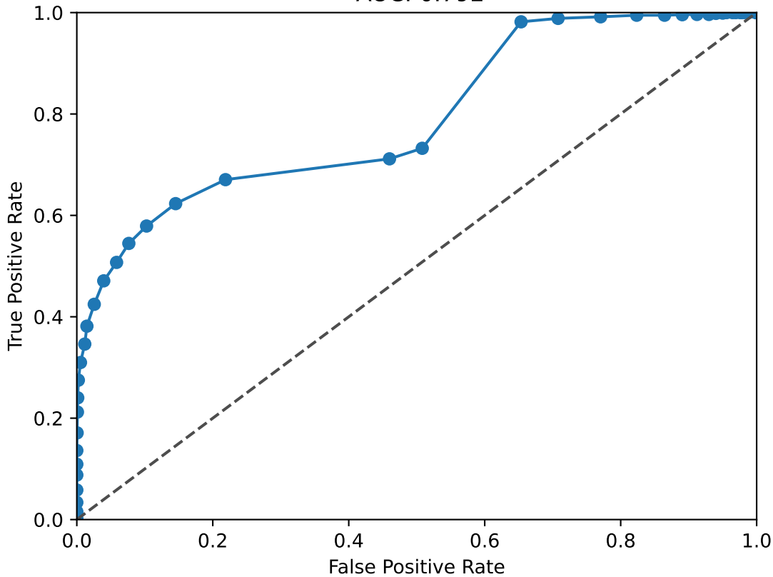
JUNB ROC Curve AUC: 0.792
