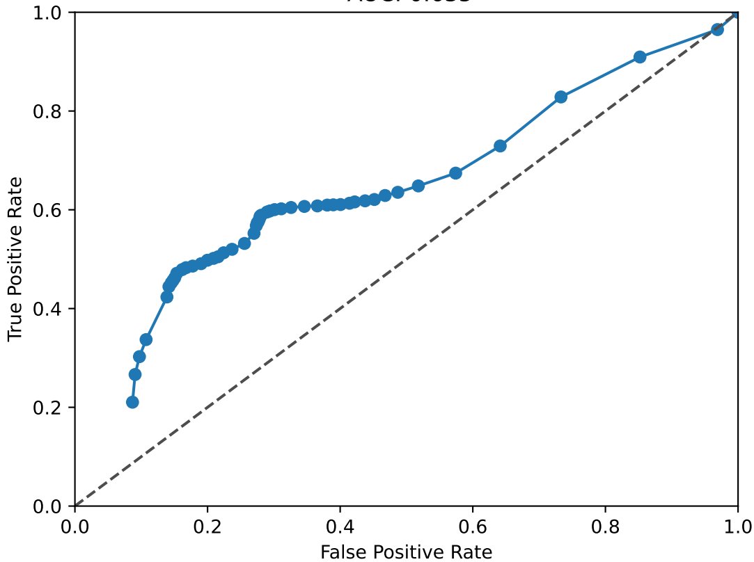
NFIX ROC Curve AUC: 0.635
