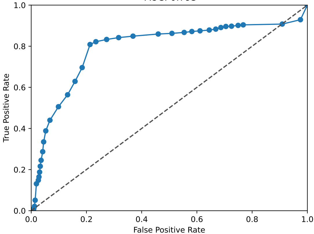
SOX11 ROC Curve AUC: 0.793
