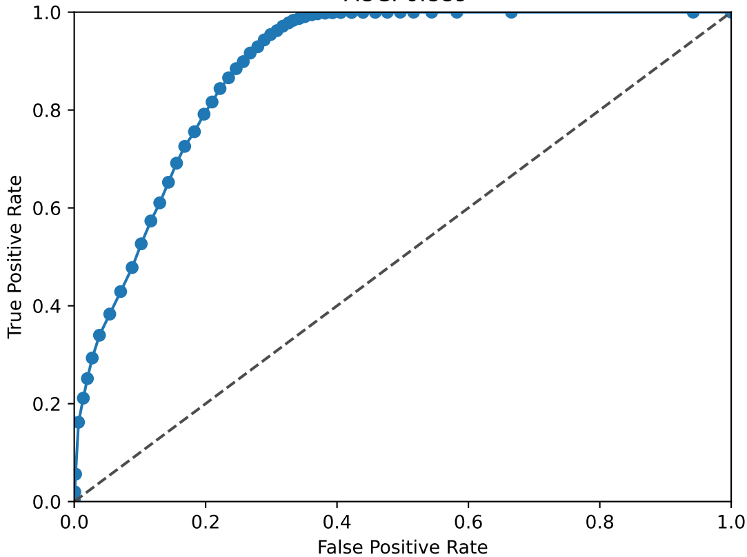
ASCL1 ROC Curve AUC: 0.889
