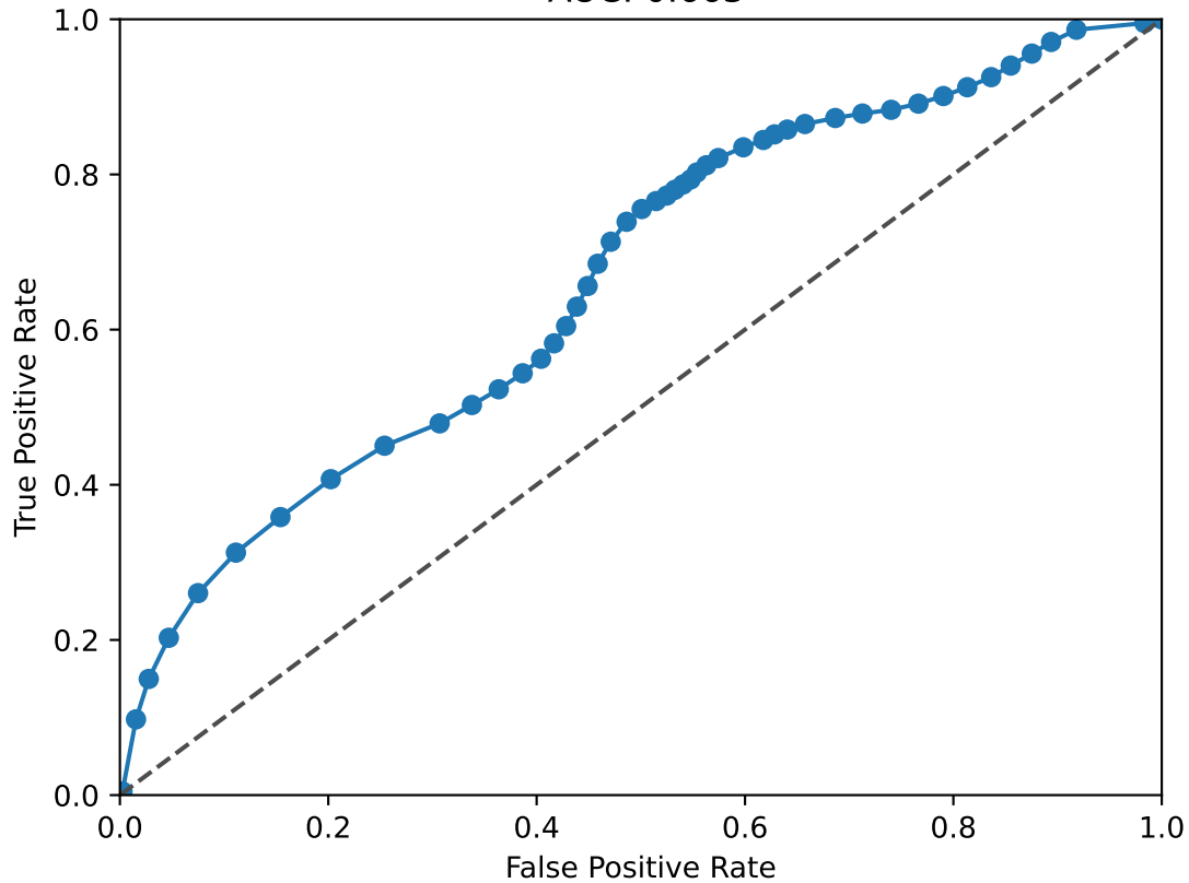
EGR1 ROC Curve AUC: 0.663
