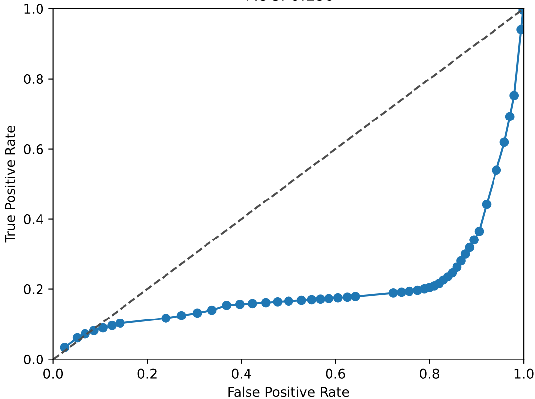
ETS1 ROC Curve AUC: 0.199
