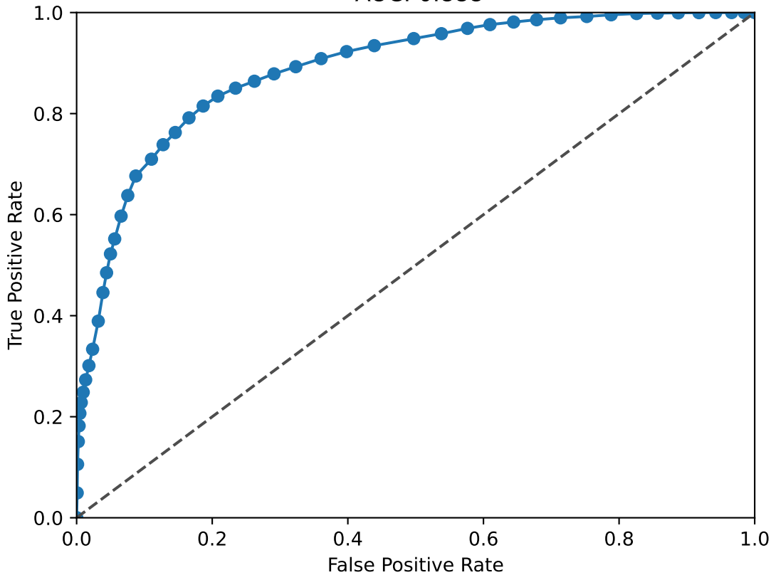
FOS ROC Curve AUC: 0.888
