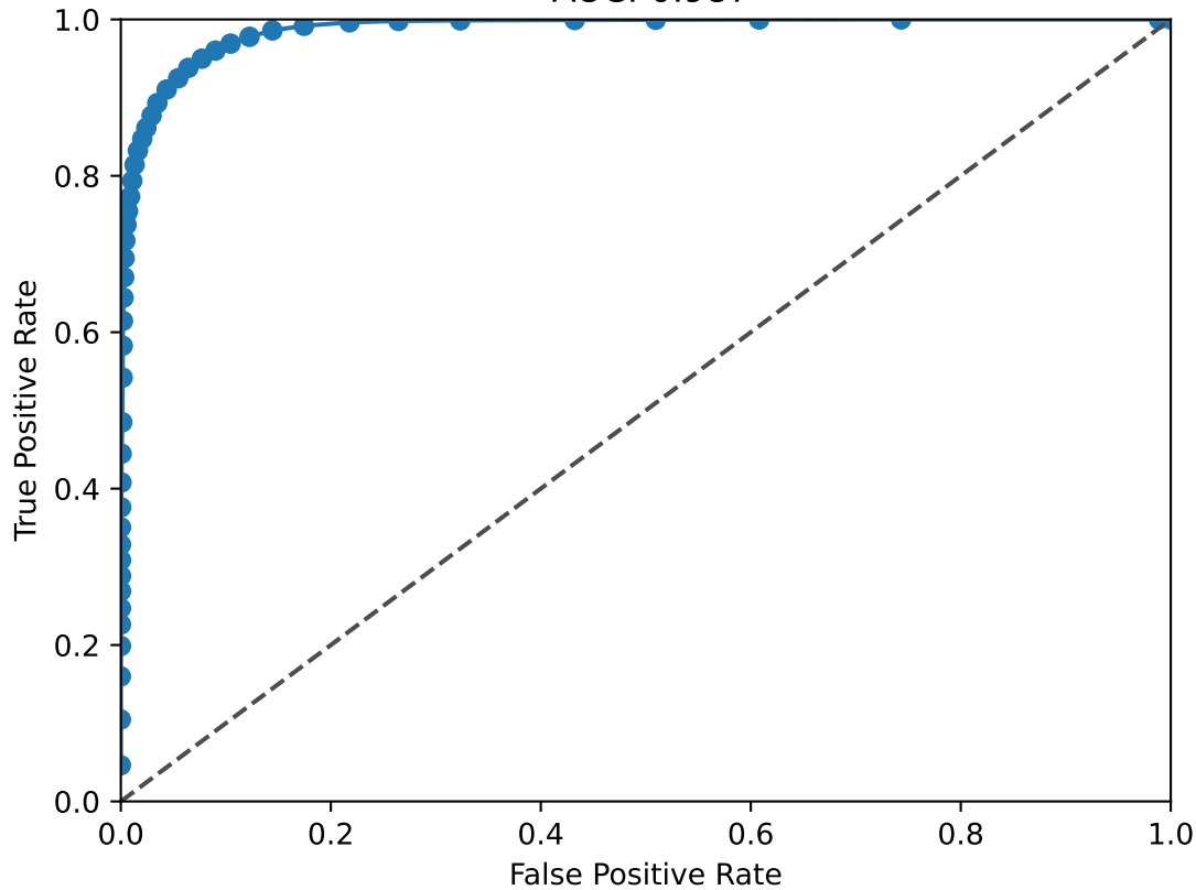
HSF2 ROC Curve AUC: 0.987
