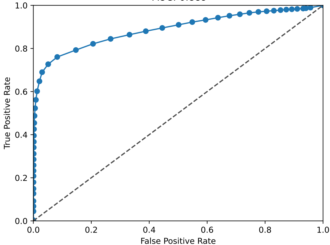
NCAM1 ROC Curve AUC: 0.889
