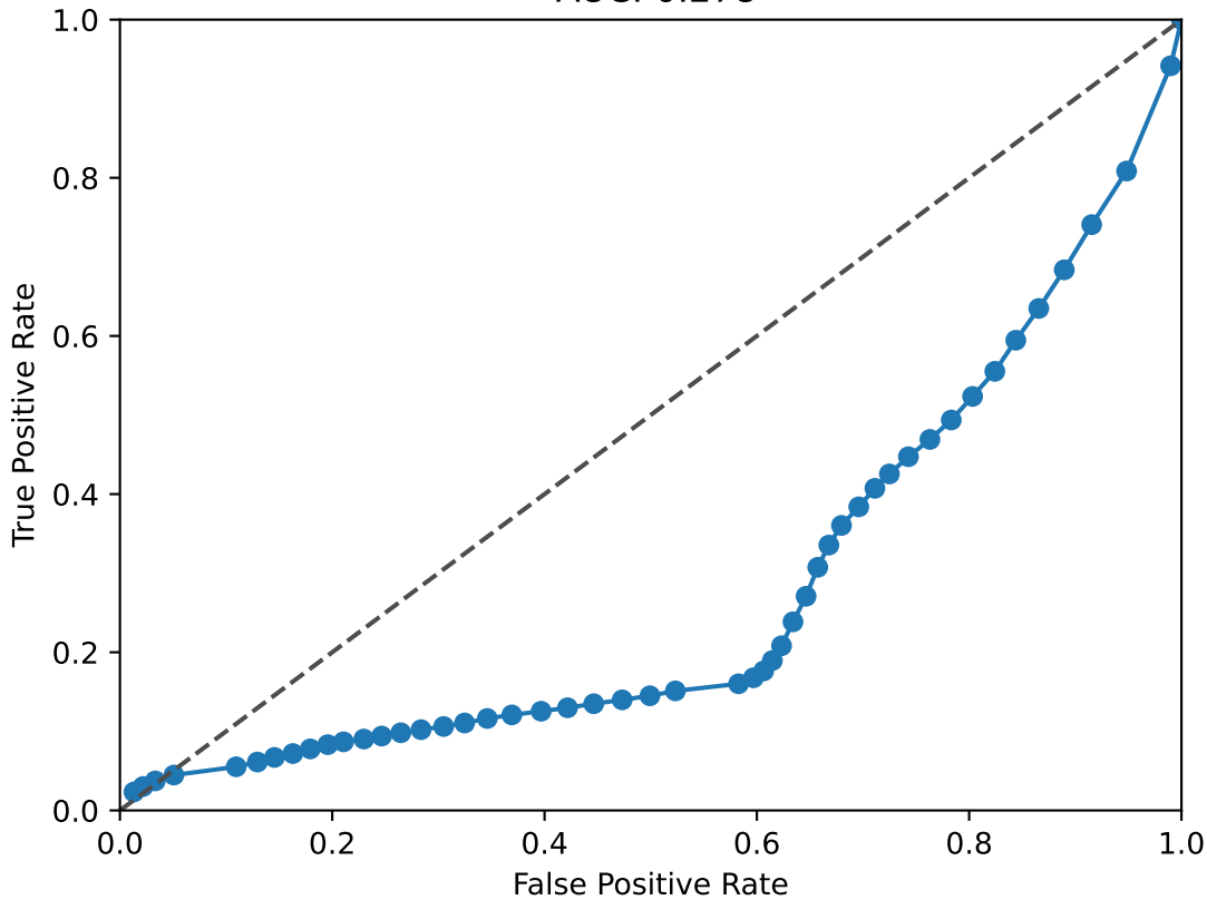
NFIX ROC Curve AUC: 0.278
