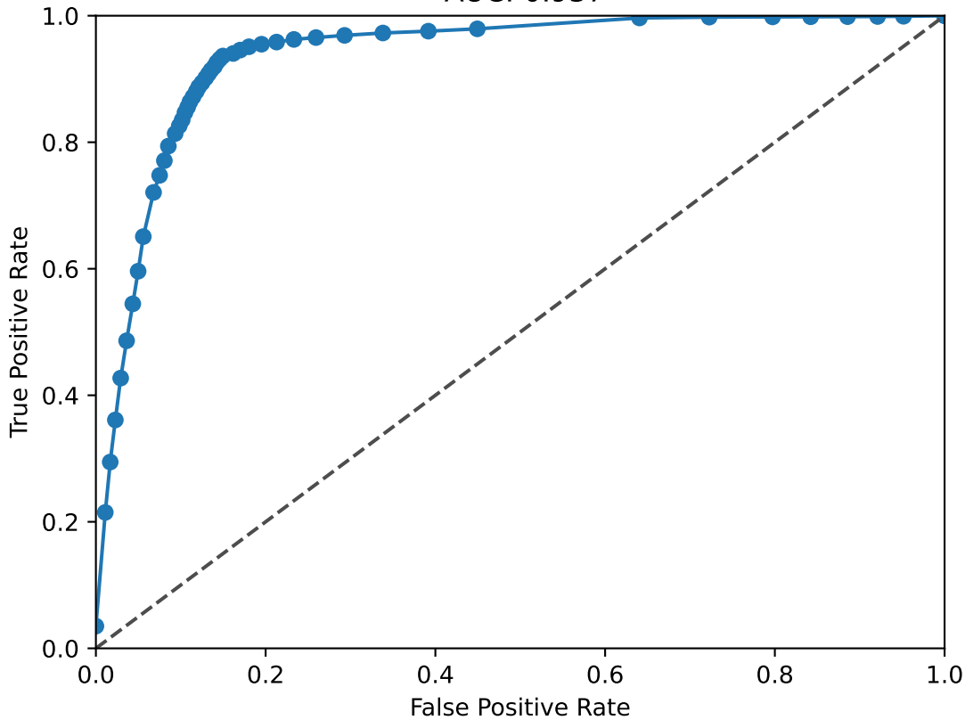
PKNOX2 ROC Curve AUC: 0.937
