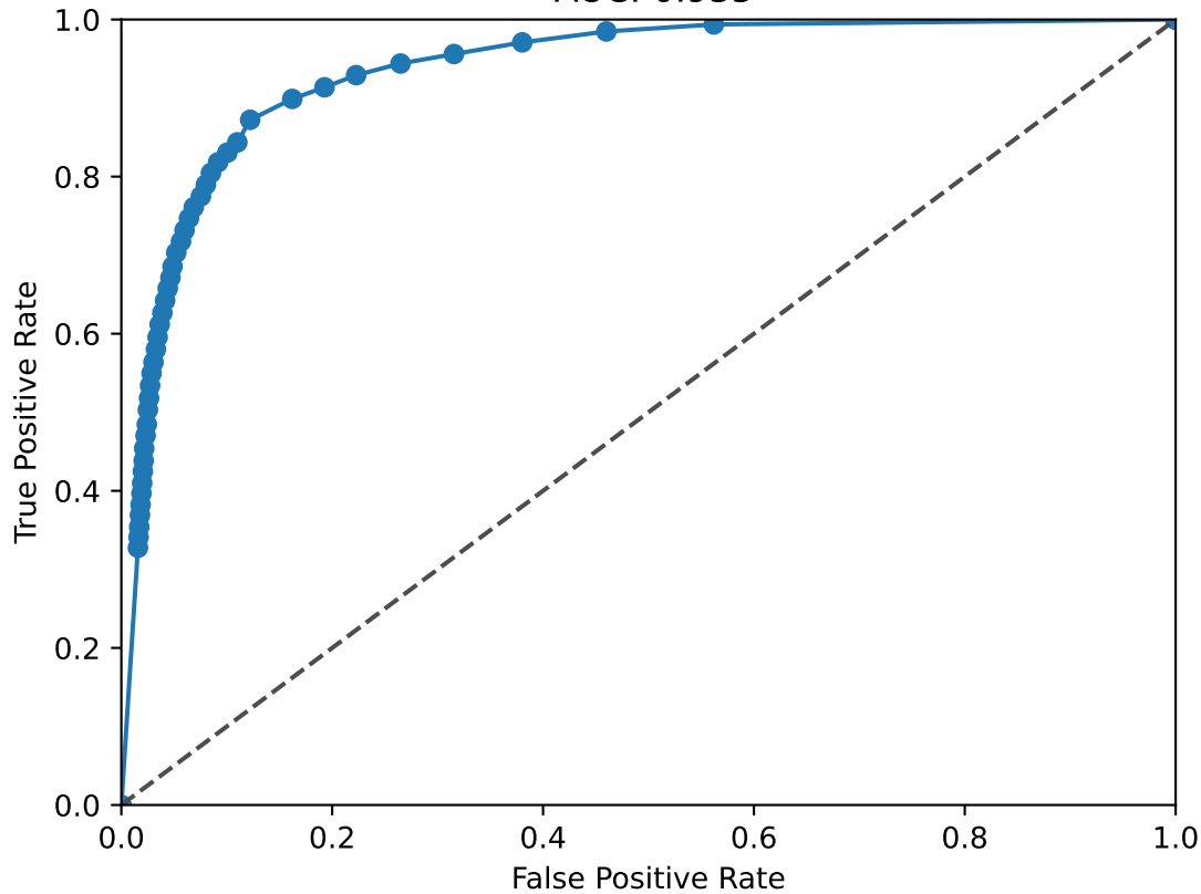
PROX1 ROC Curve AUC: 0.935
