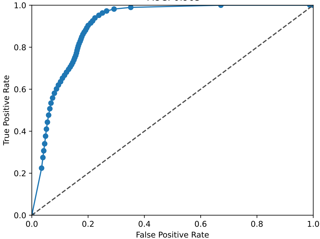
SIX1 ROC Curve AUC: 0.905
