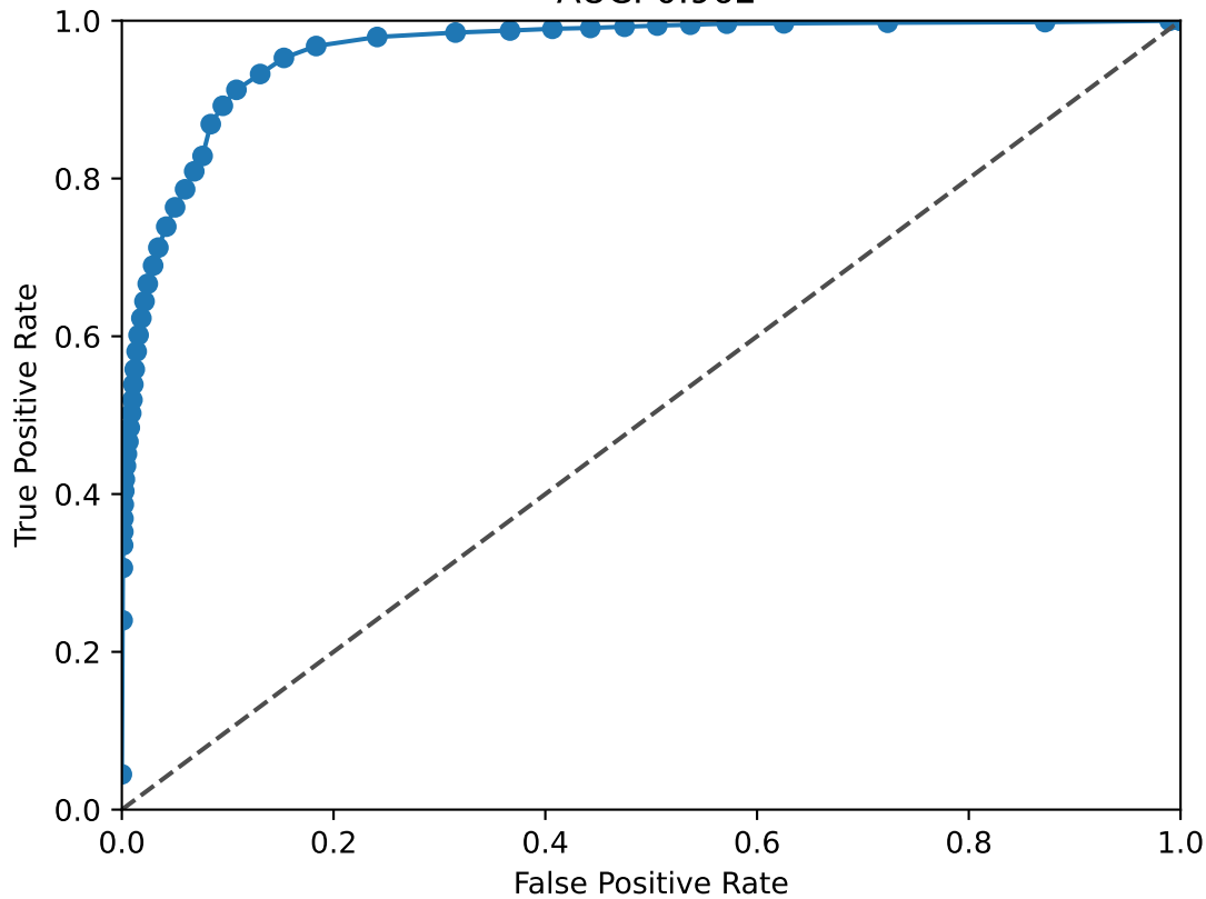
SMAD3 ROC Curve AUC: 0.962
