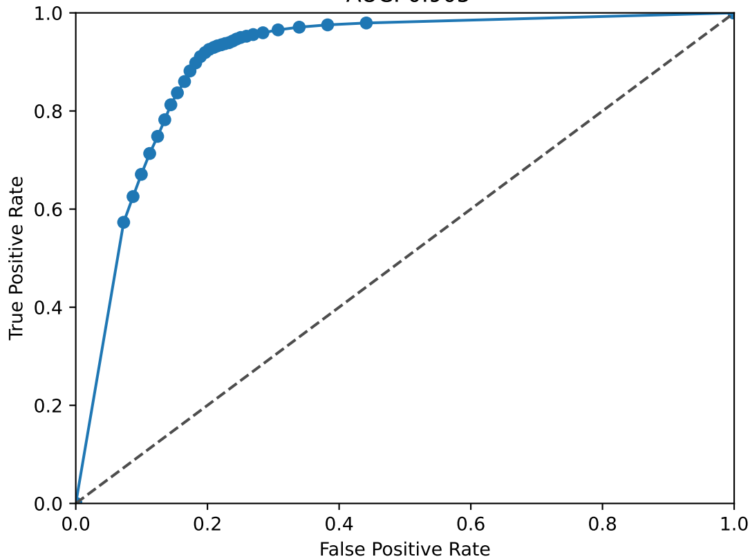
THR B ROC Curve AUC: 0.905
