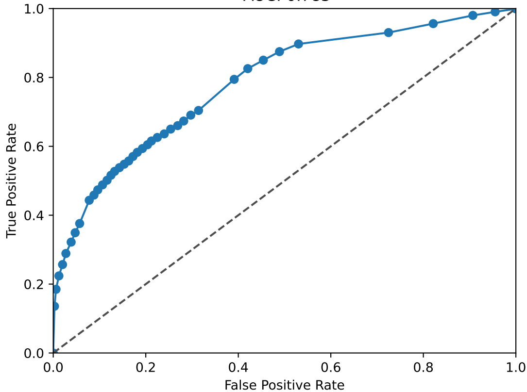
BACH2 ROC Curve AUC: 0.783
