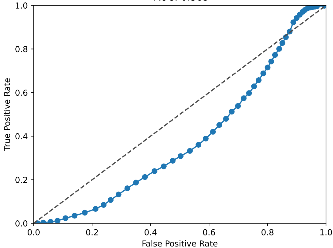
CUX2 ROC Curve AUC: 0.385
