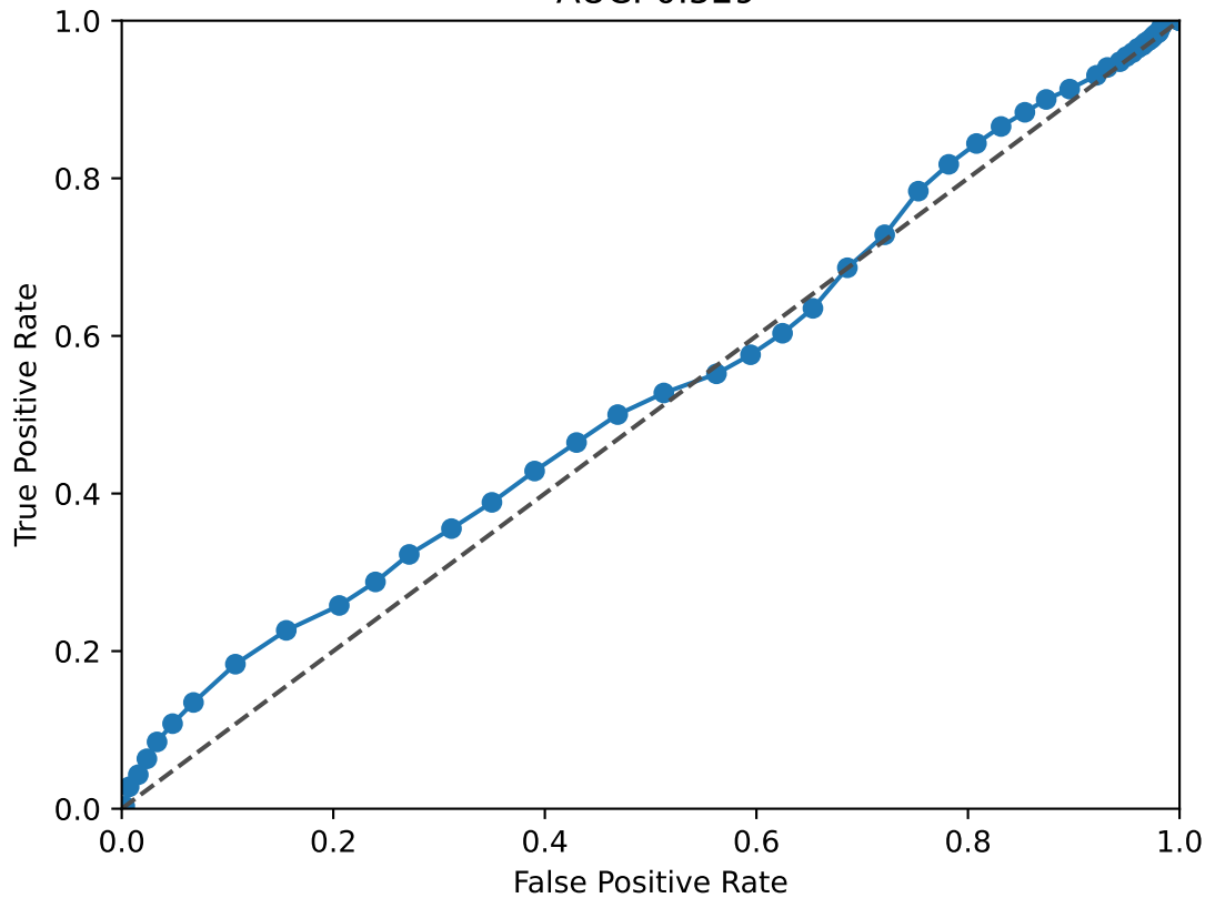
EGR1 ROC Curve AUC: 0.529
