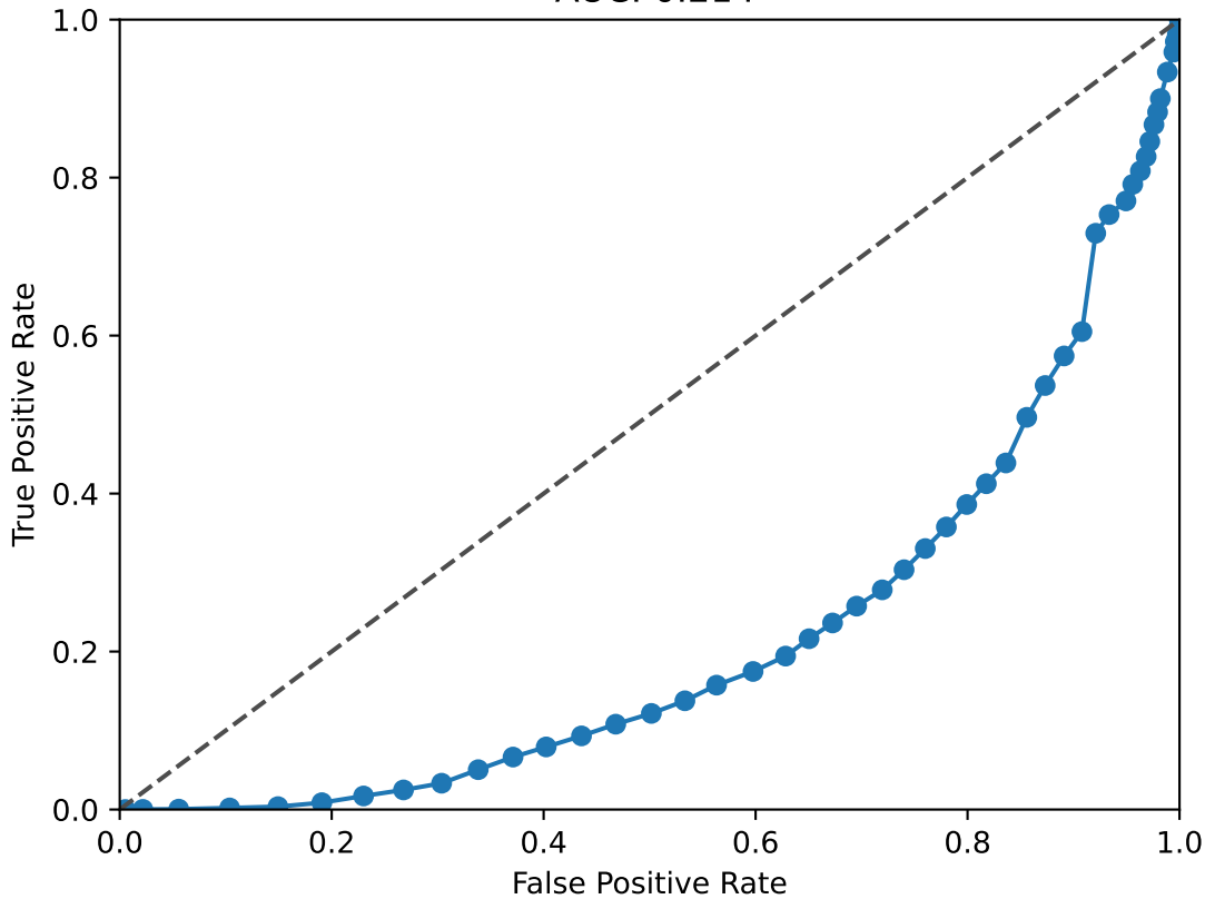
EPCAM ROC Curve AUC: 0.214
