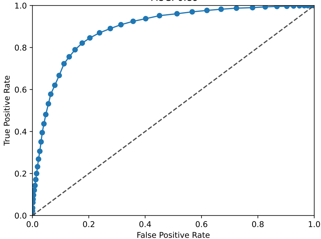
FOS ROC Curve AUC: 0.89
