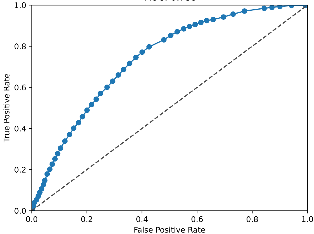
HSF2 ROC Curve AUC: 0.739
