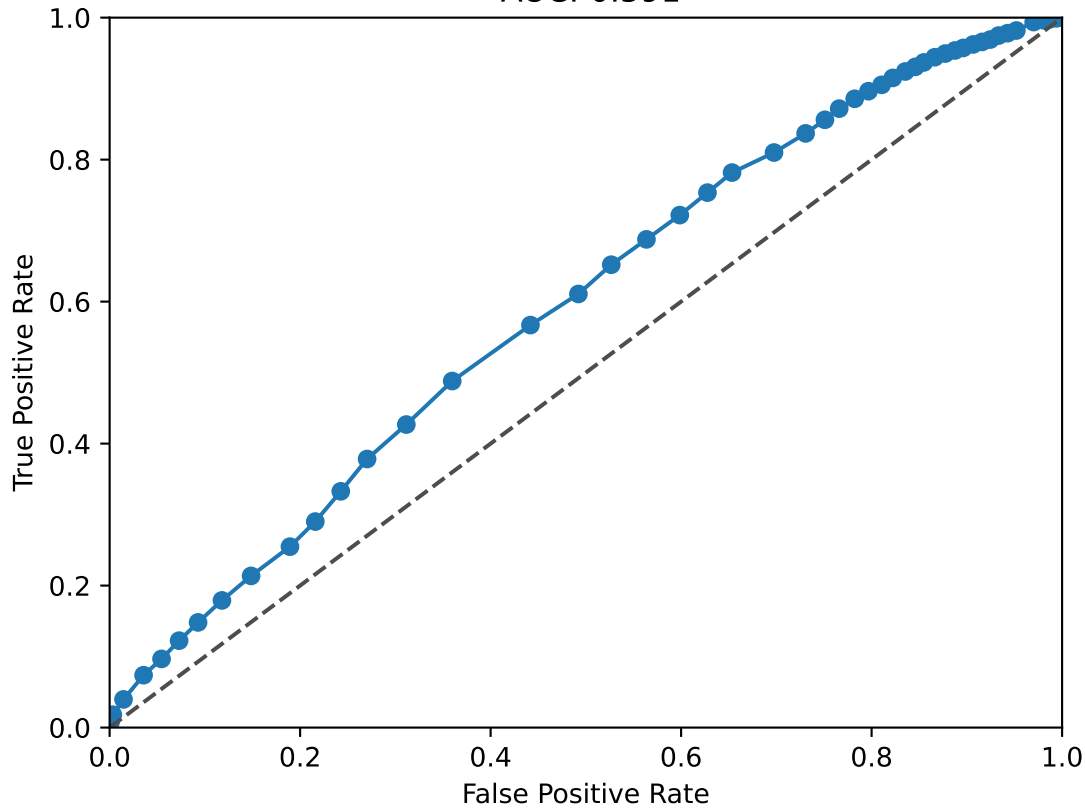
KMT2A ROC Curve AUC: 0.591
