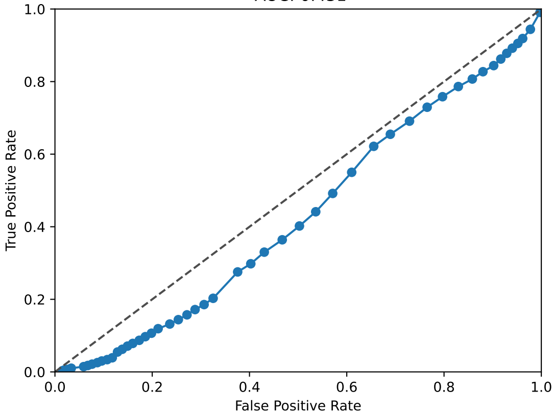
NFIX ROC Curve AUC: 0.431
