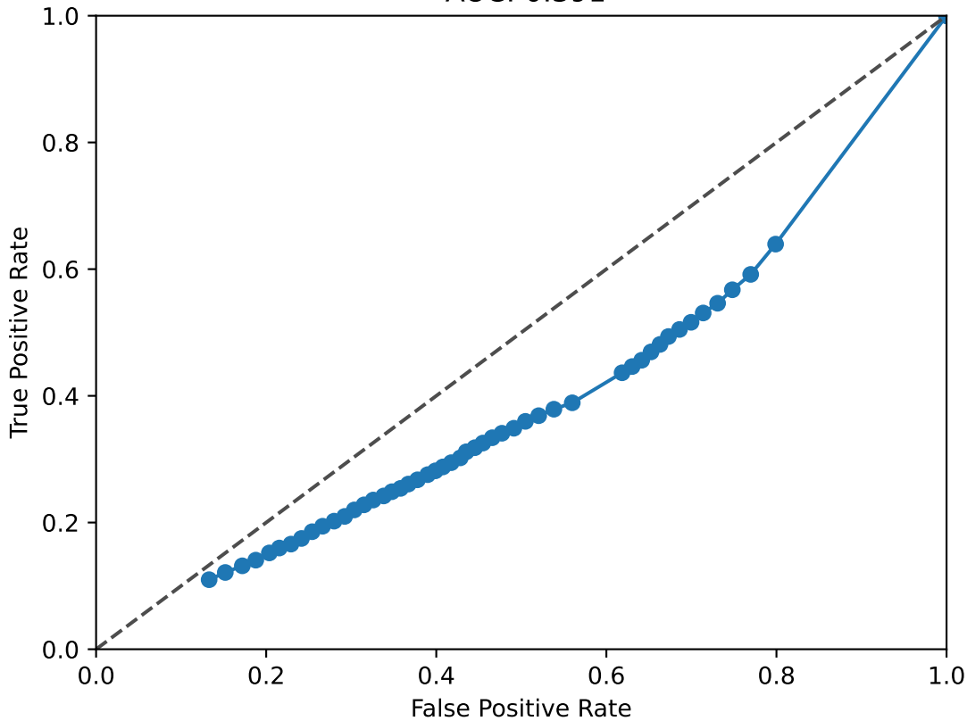
REST ROC Curve AUC: 0.391
