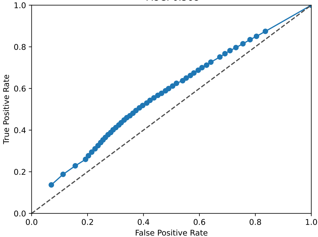
RORA_RORB ROC Curve AUC: 0.568
