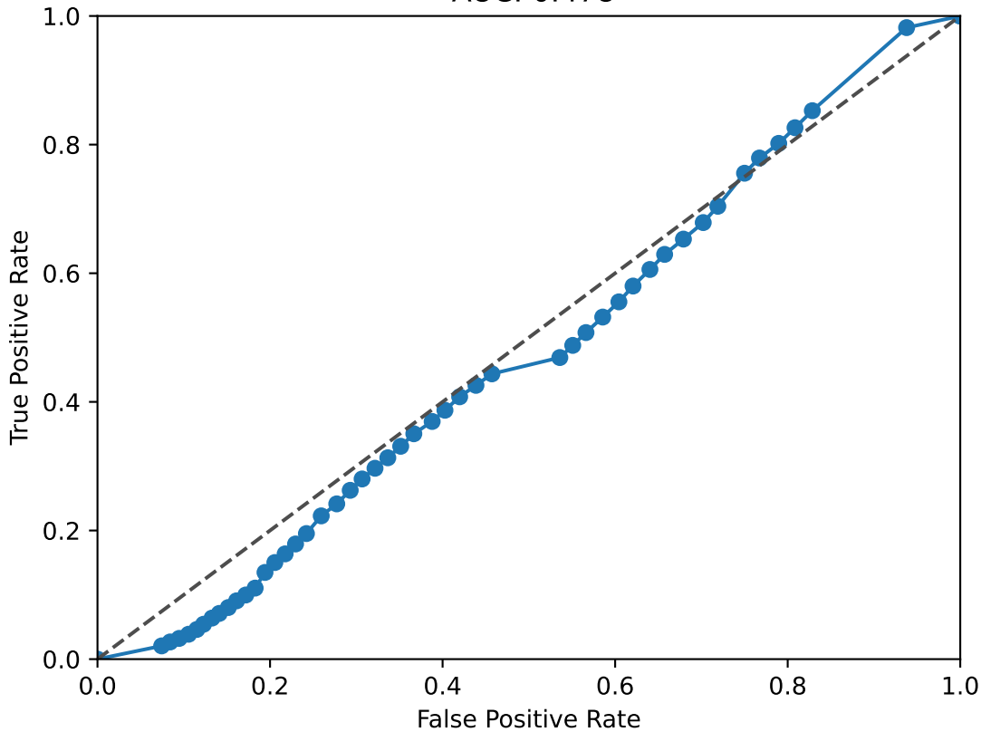
SIX1 ROC Curve AUC: 0.478
