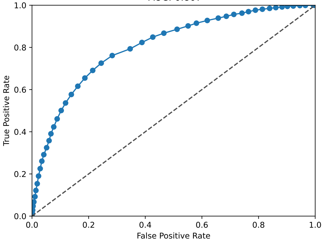
SIX4 ROC Curve AUC: 0.807
