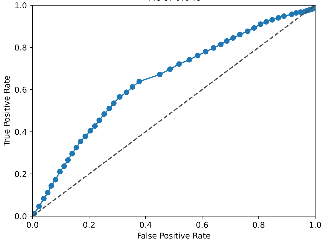
CUX2 ROC Curve AUC: 0.649
