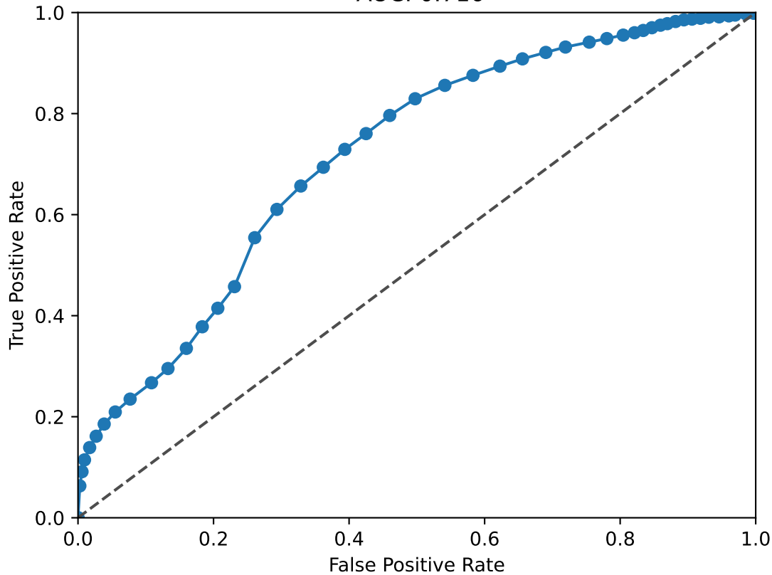
EGR1 ROC Curve AUC: 0.716
