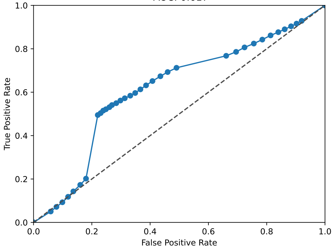
EHF ROC Curve AUC: 0.617
