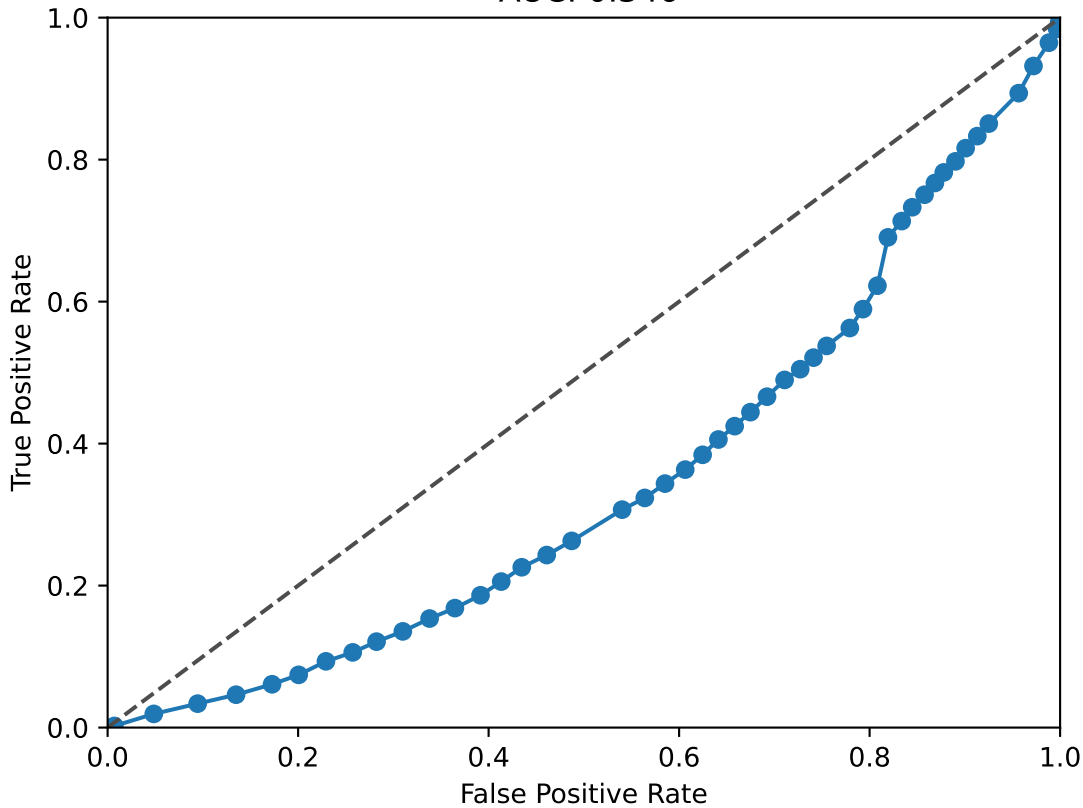
EPCAM ROC Curve AUC: 0.346
