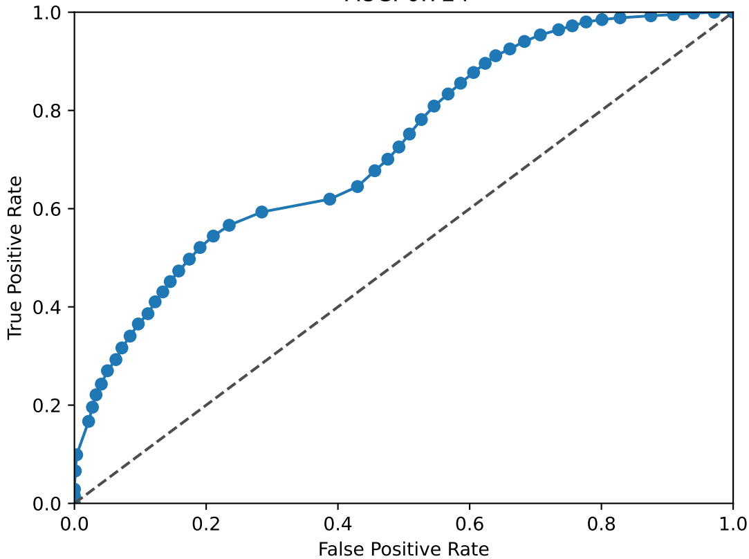
NFIB ROC Curve AUC: 0.724
