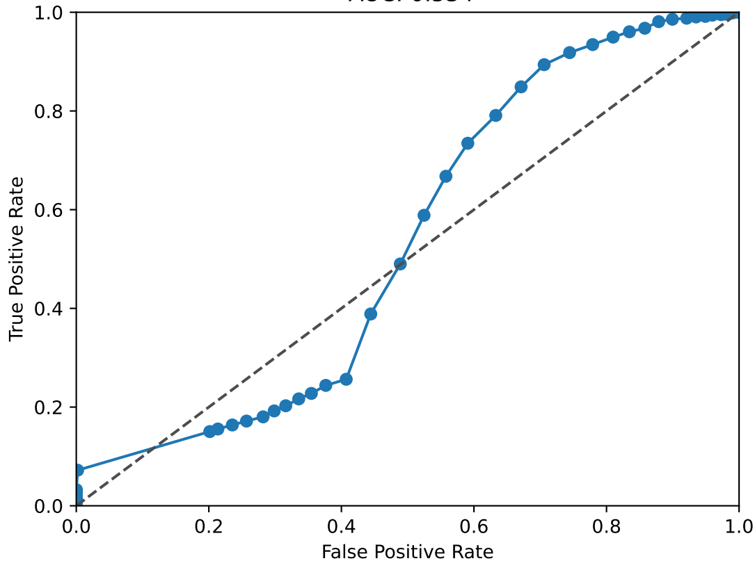
PBX1 ROC Curve AUC: 0.534
