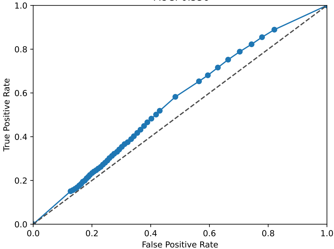
PROX1 ROC Curve AUC: 0.556
