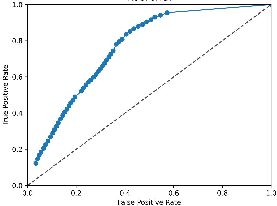
REST ROC Curve AUC: 0.757
