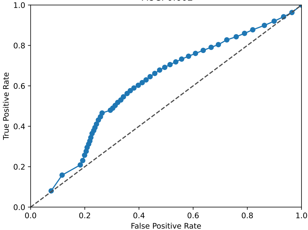
RORA_RORB ROC Curve AUC: 0.602
