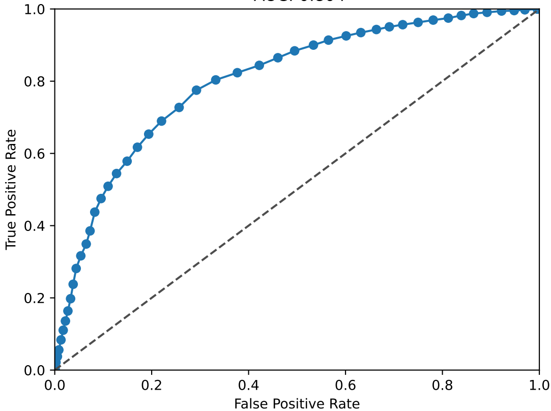
SIX4 ROC Curve AUC: 0.804
