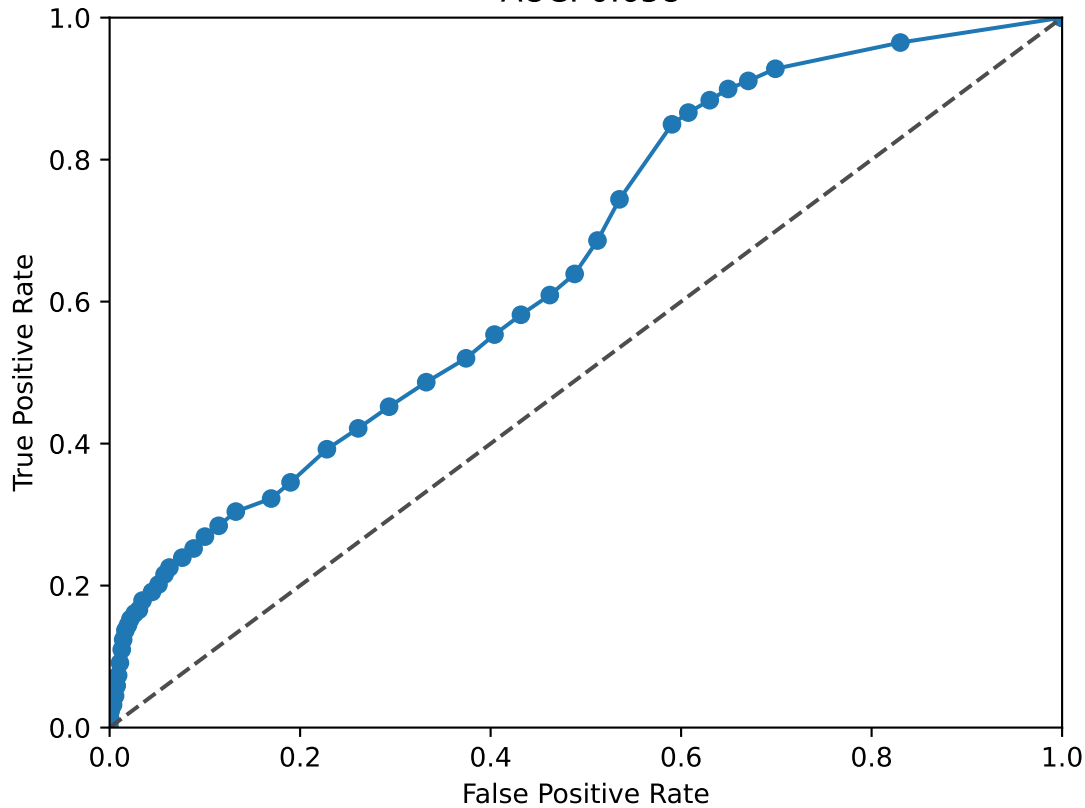
SOX11 ROC Curve AUC: 0.658
