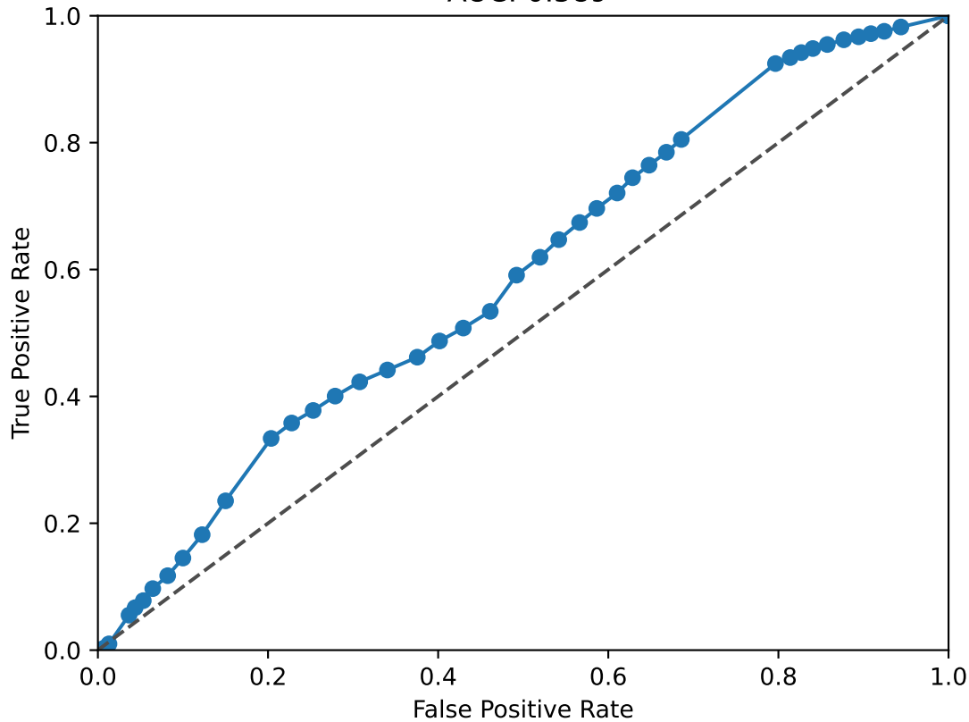
STAT2 ROC Curve AUC: 0.589
