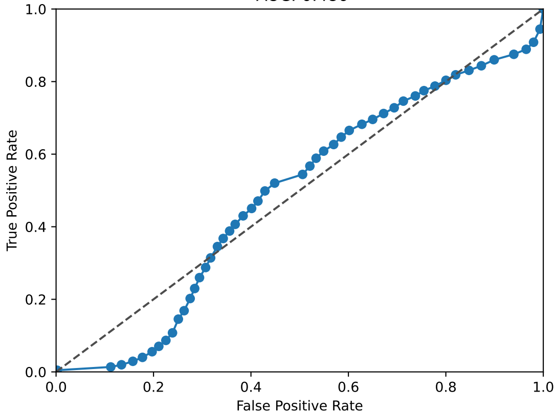
TBX15 ROC Curve AUC: 0.486
