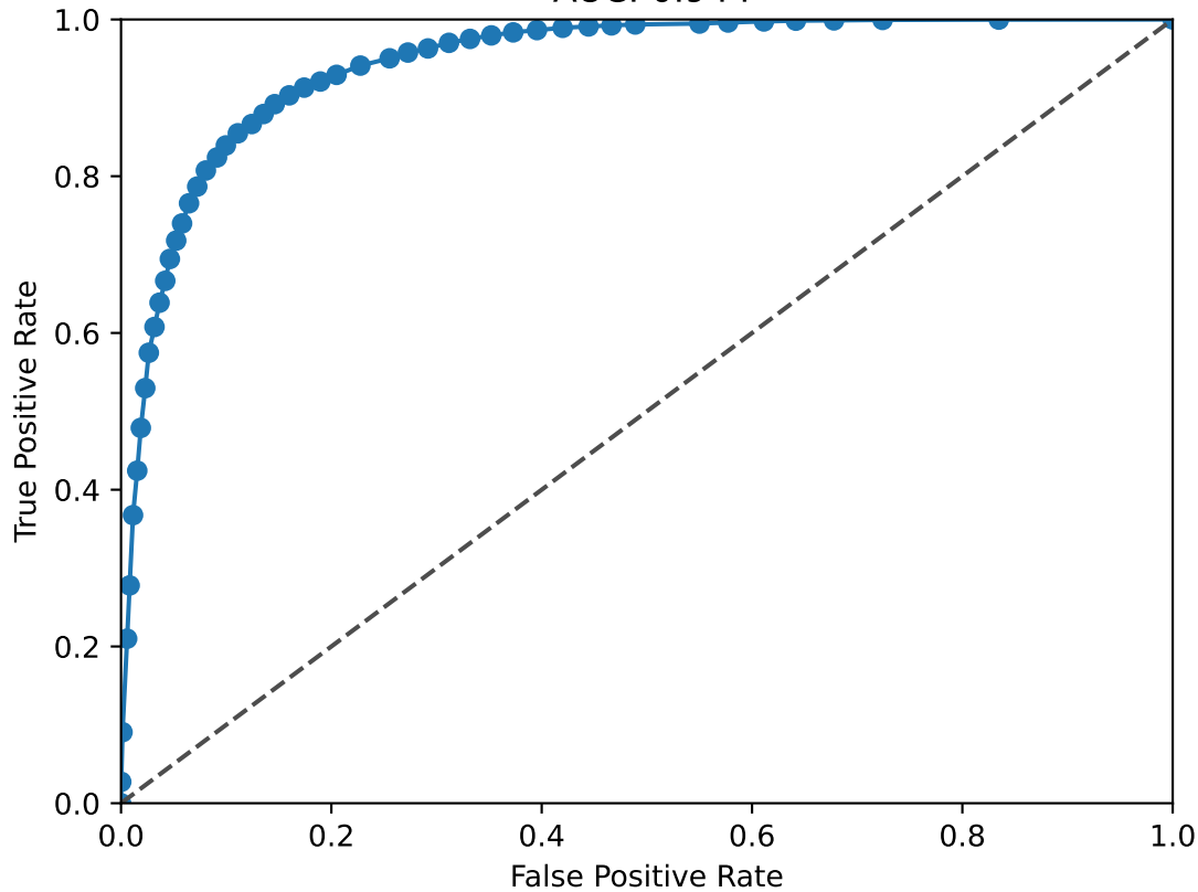
TEAD1 ROC Curve AUC: 0.944
