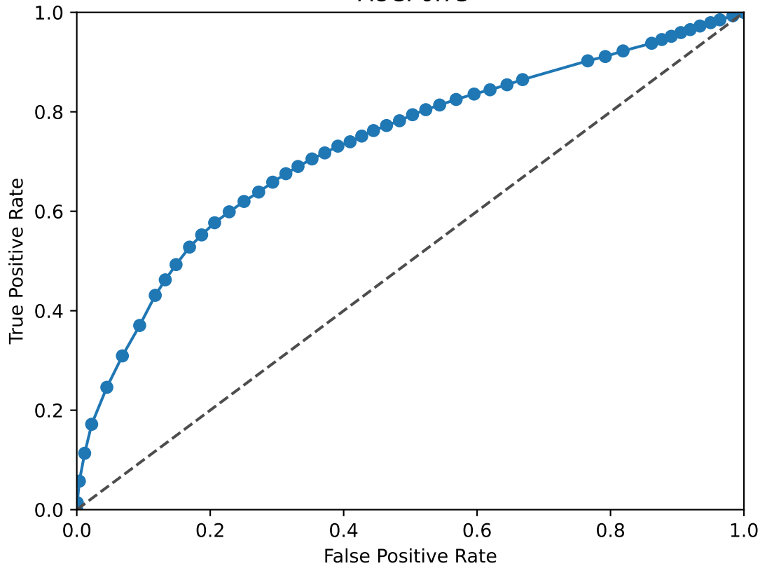
BACH1 ROC Curve AUC: 0.73
