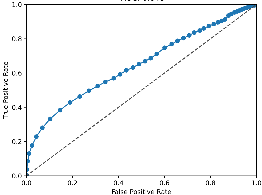
EGR1 ROC Curve AUC: 0.648
