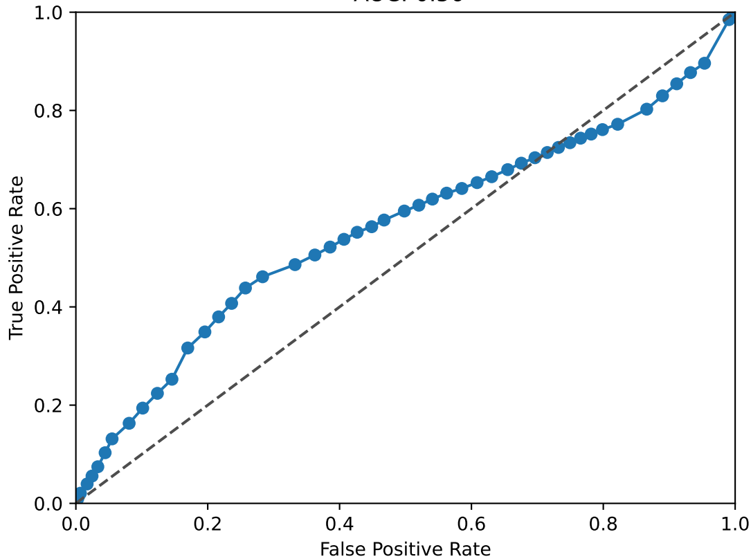
ETS1 ROC Curve AUC: 0.56
