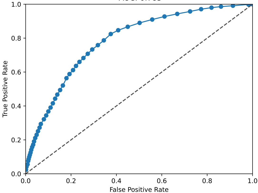
ICAM1 ROC Curve AUC: 0.783
