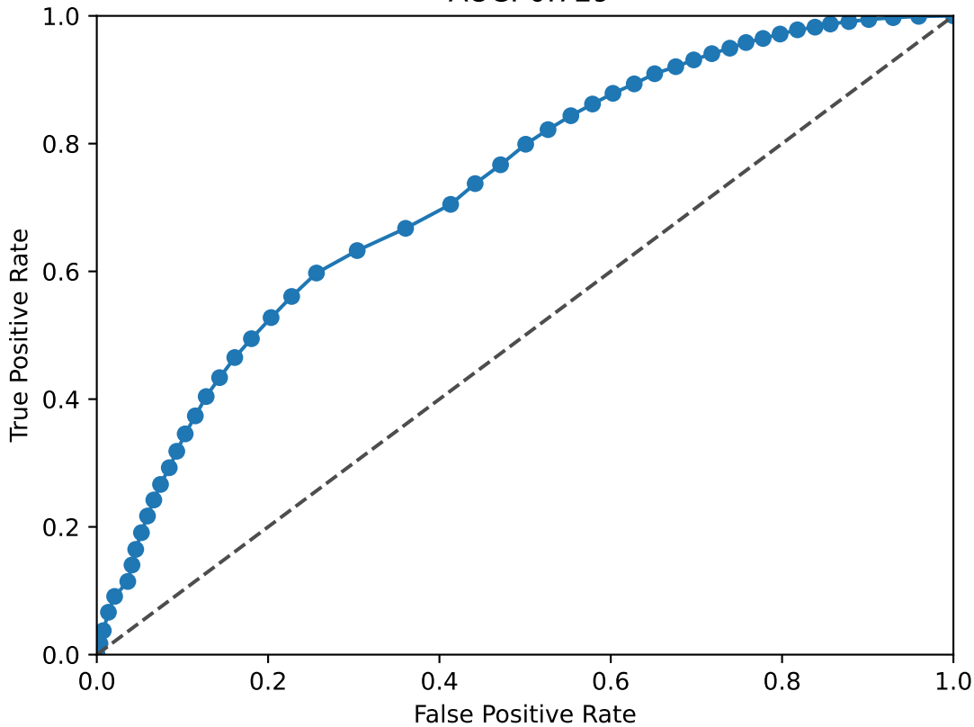
NFIB ROC Curve AUC: 0.729
